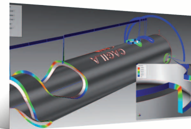
tool path analysis
