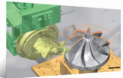
3D simulation of laser tool path
