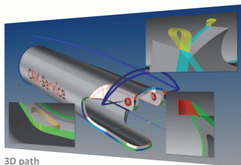
3D path optimization by destruction loops, leads, sky writing, etc.
